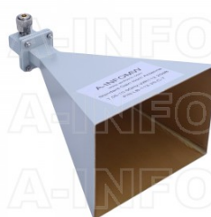
LB-112-20-C-7 Standard Gain Horn Antenna 7.05-10GHz 20dB Gain 7mm
